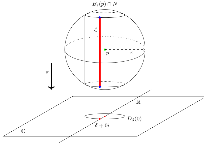
Fig. 1.4 Normal slice with complex link, \epsilon -ball and \delta -disk
