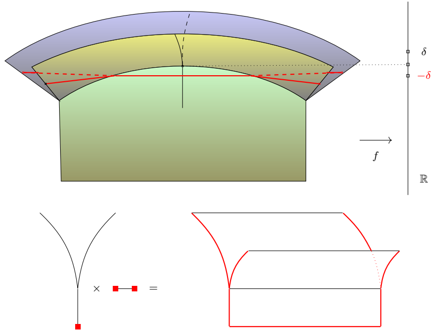
Fig. 1.3 Normal Morse data \times Tangntial Morse data = Total Morse data Glue along the red subspace
