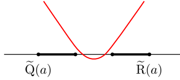
FIGURE 4. Disconnected spectrum and non-negative non-monotone curve
