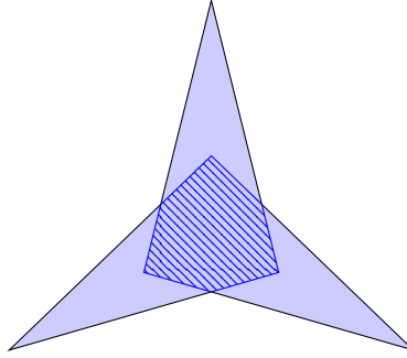
FIGURE 2. Example of a star-convex set (blue filled region) that is not convex. The subset of centers (striped region) is always convex.
