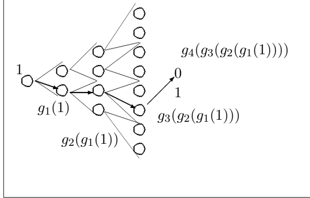
Figure 1: TPJ function ( k = 4, m = 1, d = 2 ).
