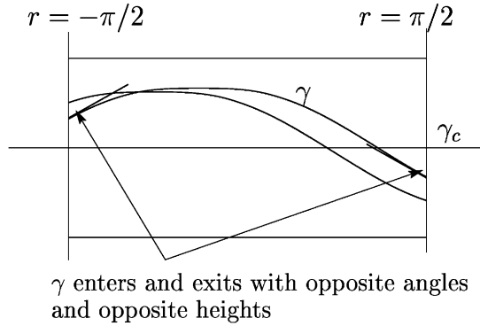
Fig. 10. The rectangle A_p (corresponding to zone A). Metric (31) is the standard metric on S^2 .
