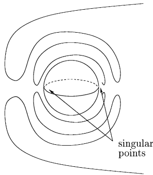
Fig. 2. The singular lamination in half of a neighborhood of the strictly stable 2-sphere.
