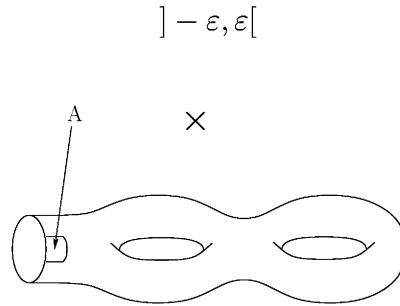
Fig. 5. Metric on the product of an interval with a genus g surface with a cylindrical end.
