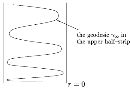
Fig. 3. The upper half-strip with the degenerate metric (4) where \lambda(r) = \cosh(\epsilon r) .
