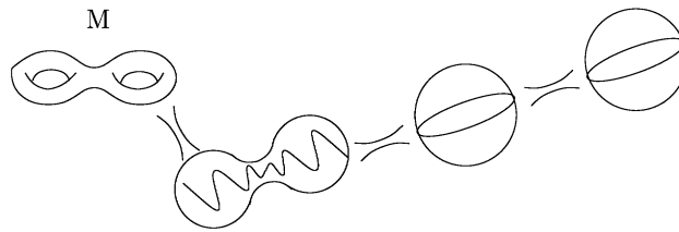
Fig. 8. Connected sum of one-parameter families of tori in g 3-spheres with the desired degeneration and M .
