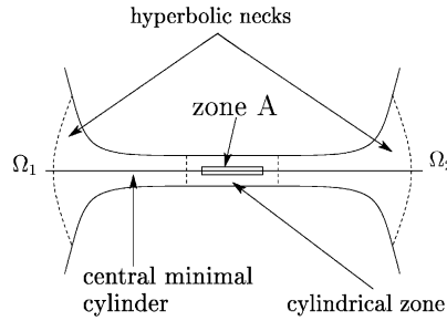
Fig. 9. The connected sum construction.
