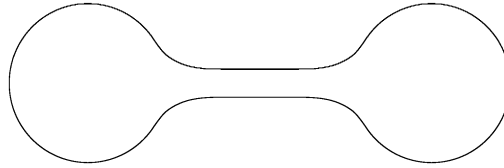
Fig. 7. The connected sum of two round S^3 's. The resulting metric has positive scalar curvature.
