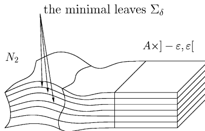
Fig. 6. Gluing together the minimal foliation of N_2 and the minimal foliation of N_1 .
