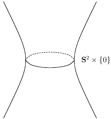
Fig. 1. The strictly stable 2-sphere in the warped metric (2) with \lambda(r) = \cosh(\epsilon r) .
