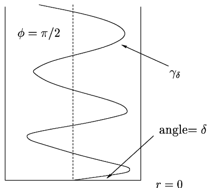
Fig. 4. The geodesic \gamma_\delta in the same half-strip.
