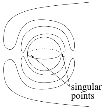
FIGURE 0.1. One of the two possible singular laminations in half of a neighborhood of a strictly stable 2-sphere. There are two leaves, namely, the strictly stable 2-sphere and half of a cylinder. The cylinder accumulates towards the 2-sphere through catenoid-type necks. In fact, the lamination has two singular points over which the necks accumulate.
