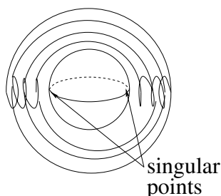
FIGURE 0.2. One of the two possible singular laminations in half of a neighborhood of a strictly stable 2-sphere. There are two leaves, namely, the strictly stable 2-sphere and half of a cylinder. The cylinder accumulates towards the 2-sphere and is obtained by gluing together two oppositely oriented double spiral staircases. Each double spiral staircase winds tighter and tighter as it approaches the 2-sphere and thus never actually reaches the 2-sphere.
