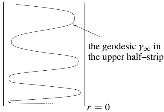
FIGURE 1.1. The projection of the half-infinite cylinder \Sigma in M is an infinite geodesic \gamma_\infty in the upper half-strip with the degenerate metric (1.4).
