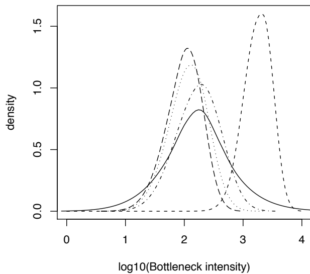
Fig. 3. Second example: posterior distributions of the bottleneck severity (see definition in text) for the invasions of four Pacific islands by Zosterops lateralis lateralis . The four discontinuous lines with small dashes, dots, dash-dots and long dashes correspond to Norfolk, Chatham, North Island and South Island of New Zealand, respectively. The continuous line corresponds to the prior distribution, which is identical for each island. This graph has been made with the locfit function of the R statistical package (Ihaka and Gentleman, 1996), using an option of DIYABC which saves the sample of the parameter values adjusted by the local linear regression (Beaumont et al., 2002).
