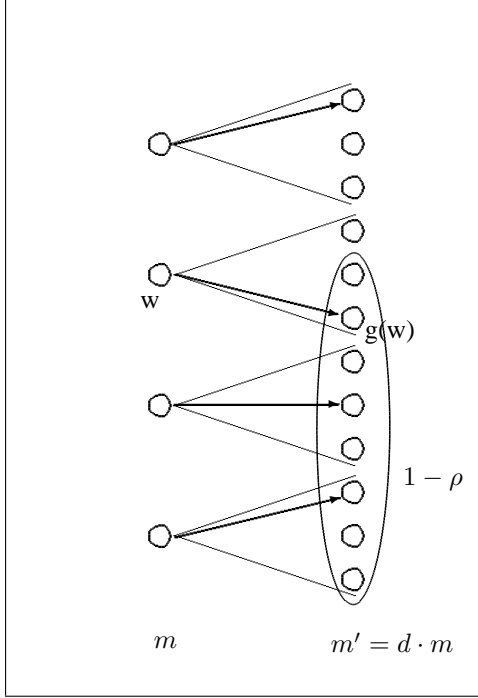
Figure 2. Variables of the proof of Th. 3.3.
