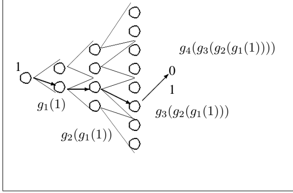
Figure 1. TPJ function ( k = 4, m = 1, d = 2 ).
